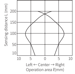
• BRP200-DDTN
